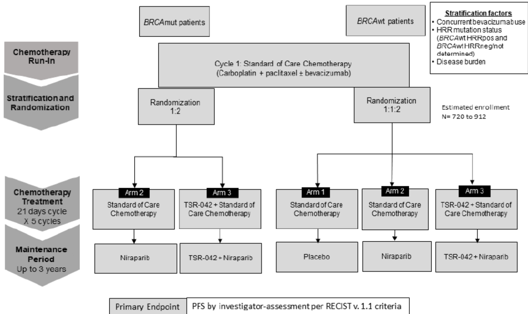
Figure 1: Study Design
